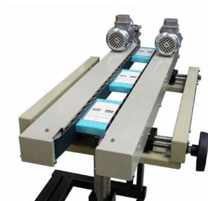
Convoyage double bandes
